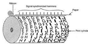
Diagram 2.27 Drum Printer
