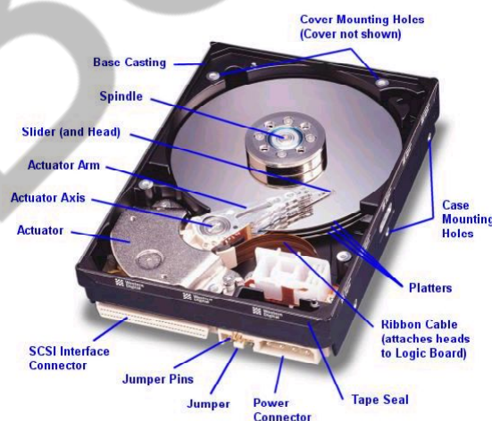
Diagram 2.3 Hard Disk
