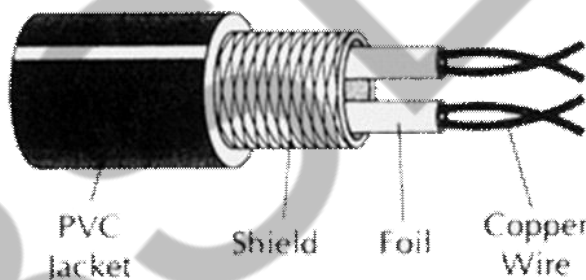
Diagram 3.4 Shielded Twisted Pair Cable
