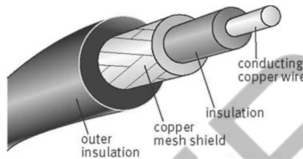
Diagram 3.5 Coaxial Cable
