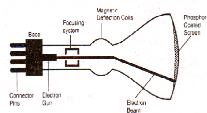
Diagram 2.22 Cathode Ray Tube
